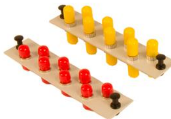
ST Simplex 8 Port plate
